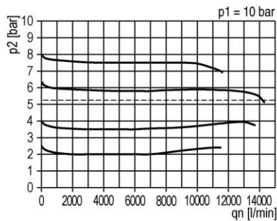
flow characteristic
