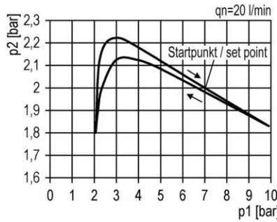
pressure characteristic
